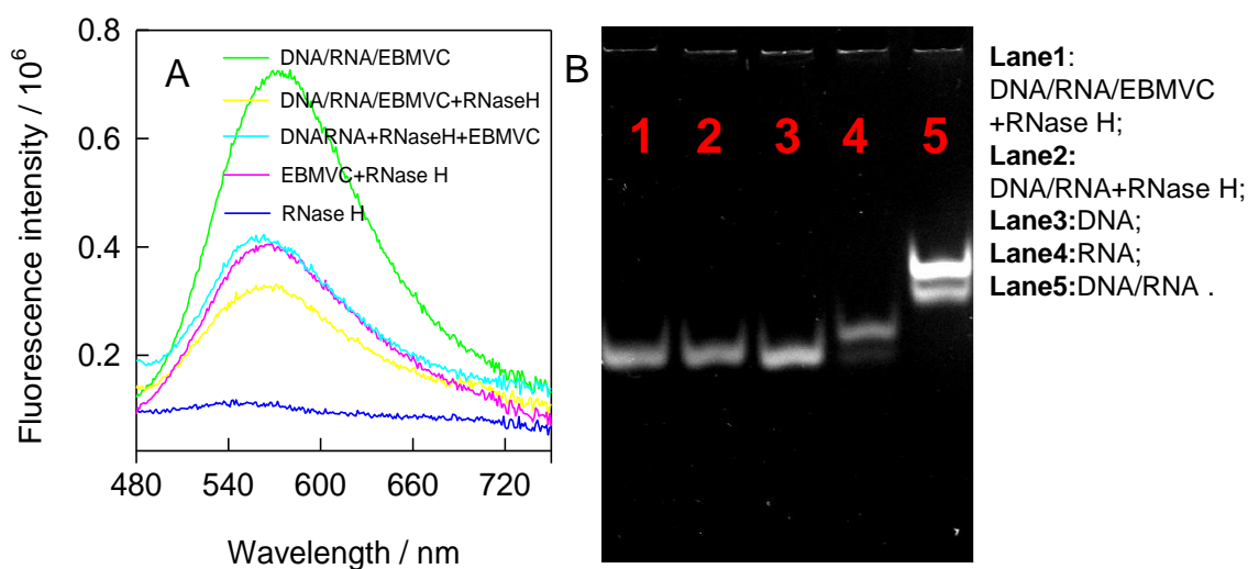
Fig. S7 A) Fluorescence emission spectra of DNA/RNA/EBMVC with/without RNase H treatment. B) Polyacrylamide gel electrophoresis, showing the disappearance of the RNA band upon treatment with RNase H for both the DNA/RNA duplex and the duplex loaded with EBMVC.
