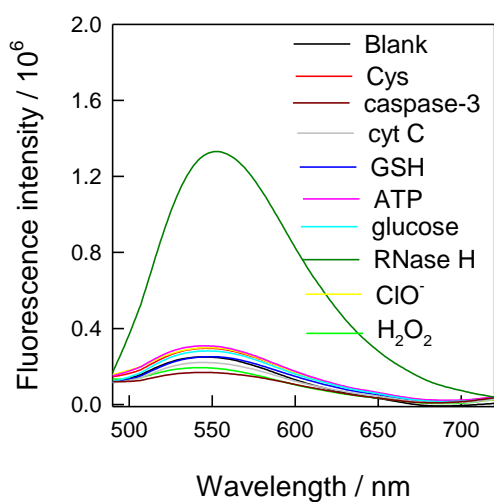
Fig. S9 Stability of the SNA probe at 37 °C to a panel of cellular species: Cys (5 mM), GSH (5 mM), ATP (10 mM), glucose (10 mM), caspase-3 (1.5 nM), Cyt C (0.28 U/mL), \text{H}_2\text{O}_2 (100 \mu\text{M} ), \text{ClO}^- (100 \mu\text{M} ), and RNase H (0.5 U/mL).
