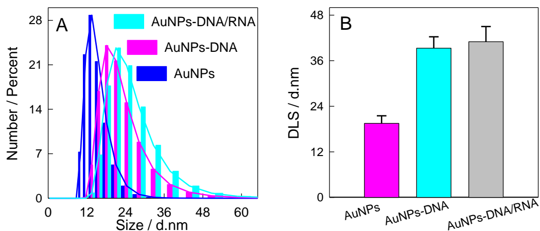
Fig. S2 Number-average size distribution (A) and Z-average size (B) measured by dynamic light scattering.
