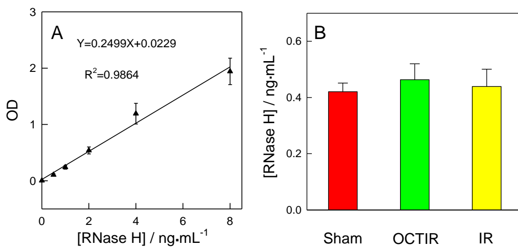
Fig. S14 Quantification of RNase H levels in rat liver tissues using ELISA. A) standard curve for RNase H, B) RNase H levels in three group rat liver tissues homogenates. Error bars were calculated from samples from three different rats.
